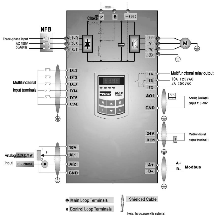
0.2kW – 22kW Basic Wiring Diagram for Multi-stage speed control macro (NPN type)
