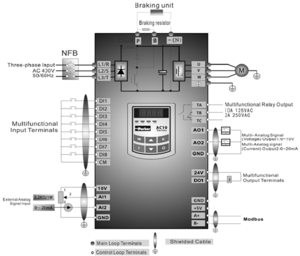
0.2kW – 22kW Basic Wiring Diagram for Multi-stage speed control macro (NPN type)
