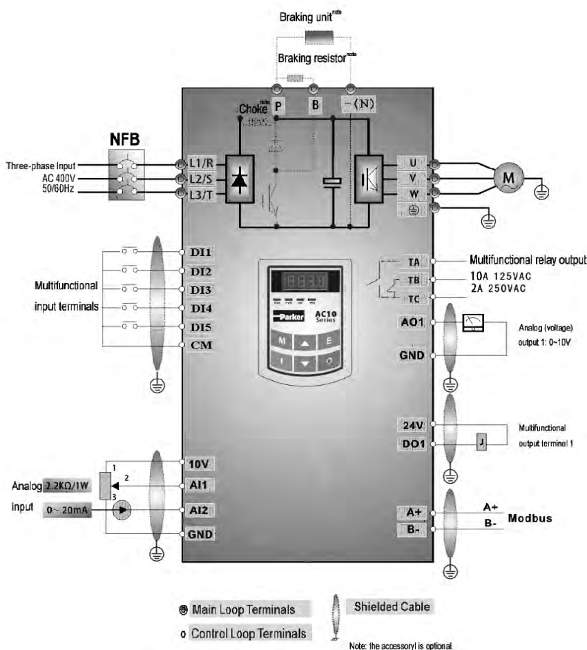
0.2kW – 22kW Basic Wiring Diagram for Multi-stage speed control macro (NPN type)
