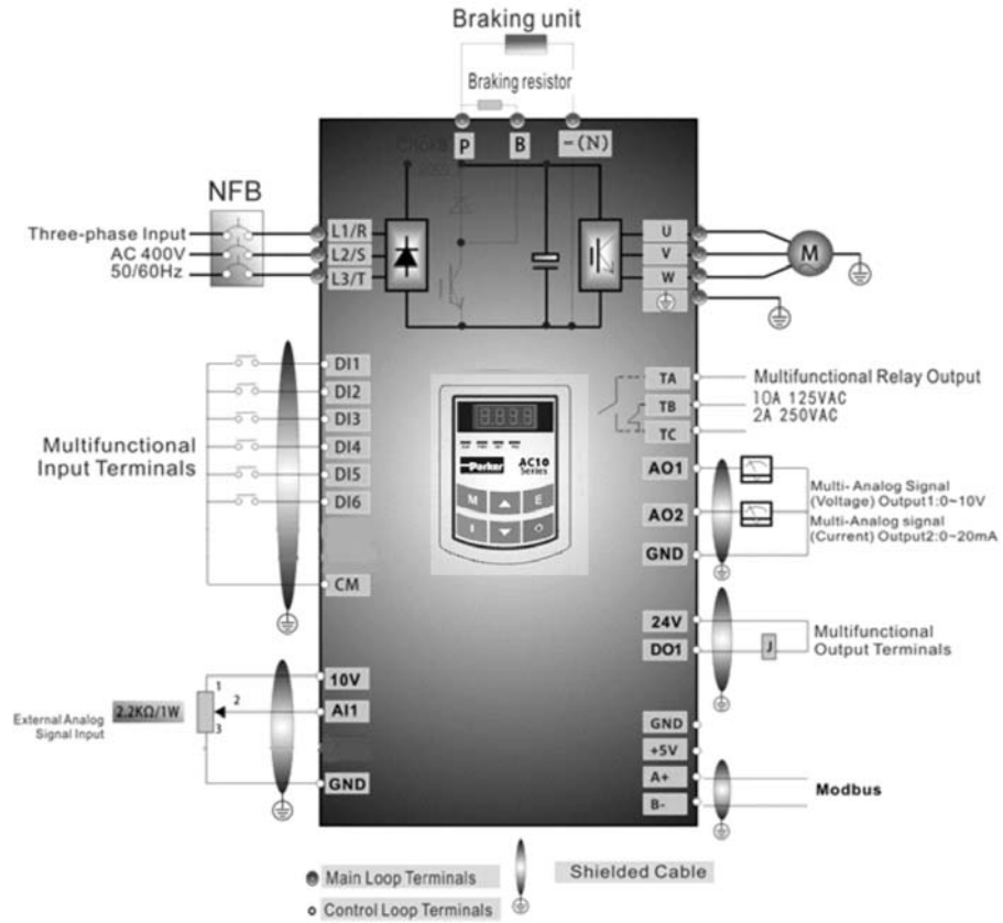
0.2kW – 22kW Basic Wiring Diagram for Multi-stage speed control macro (NPN type)
